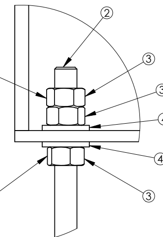
DETAIL C SCALE 1 : 2
